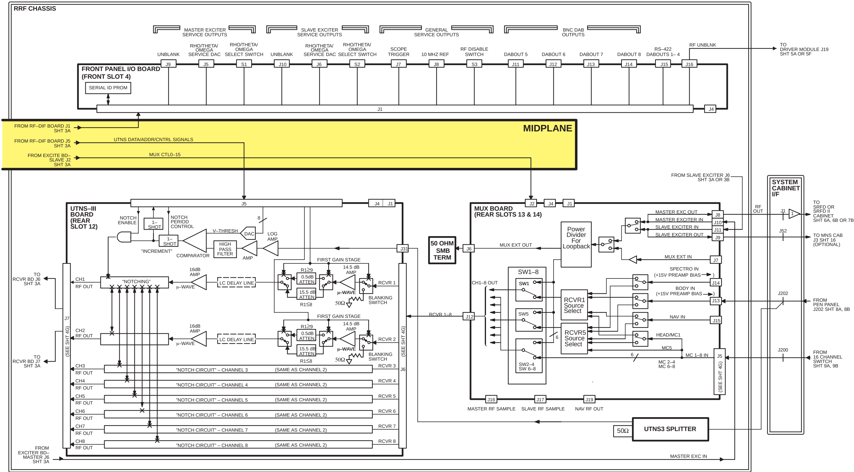
G3 & 3T94 EXCITE HD (12.x), HDx (14.x) & HDxt (15.x) MGD/RRF/RF SUBSYSTEM (8 Channel Systems) RRF CHASSIS INTERCONNECT BLOCK DIAGRAM 2 OF 2A (8 channel) SHEET 4A OF 18
