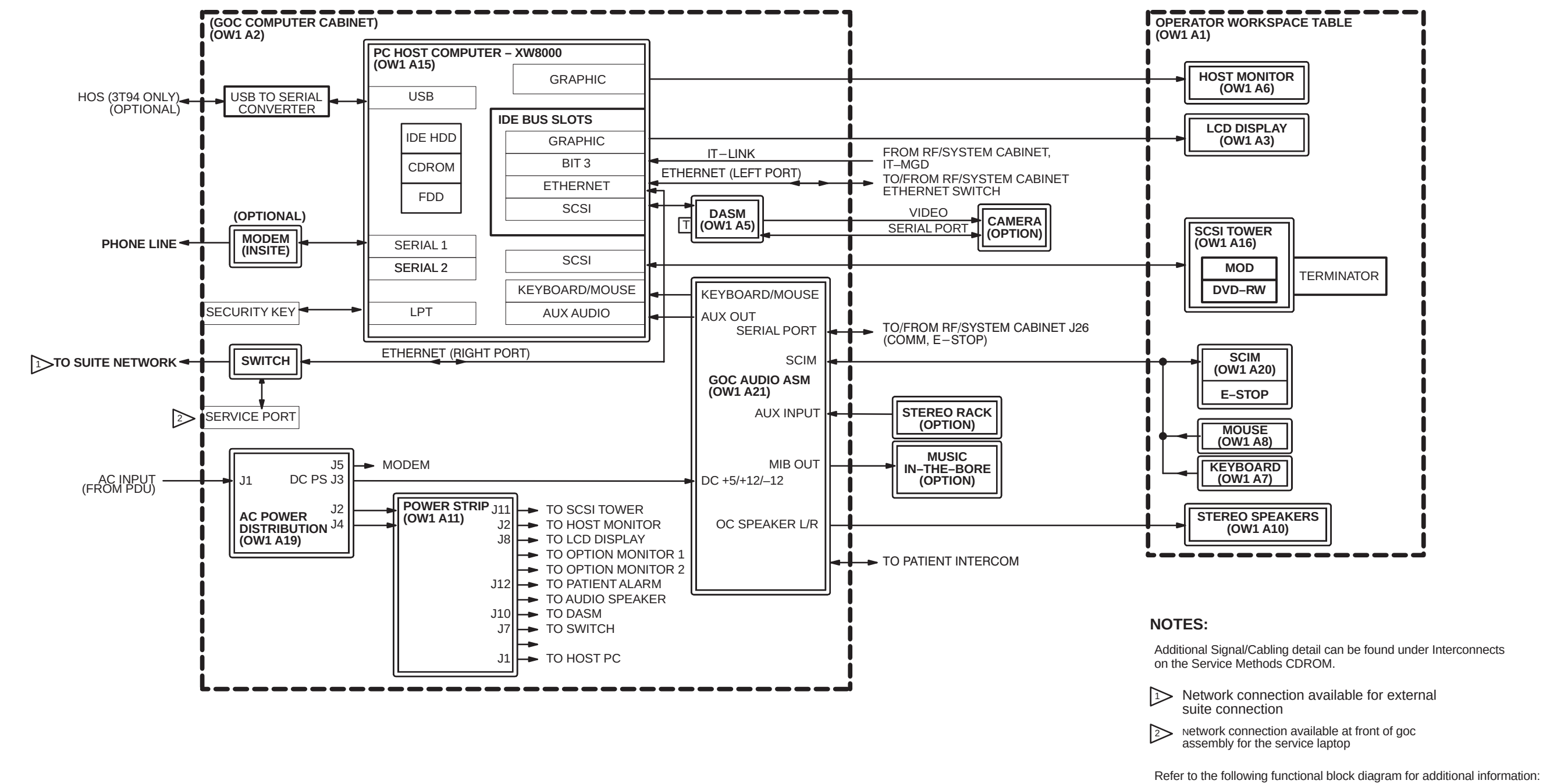
G3 & 3T94 EXCITE HD (12.x) OVERALL SYSTEM Forward Production or Pre-EXCITE Upgrades (OPERATOR WORKSPACE CABINET w/8000 & GOC AA and TABLE) SHEET 1A OF 5
