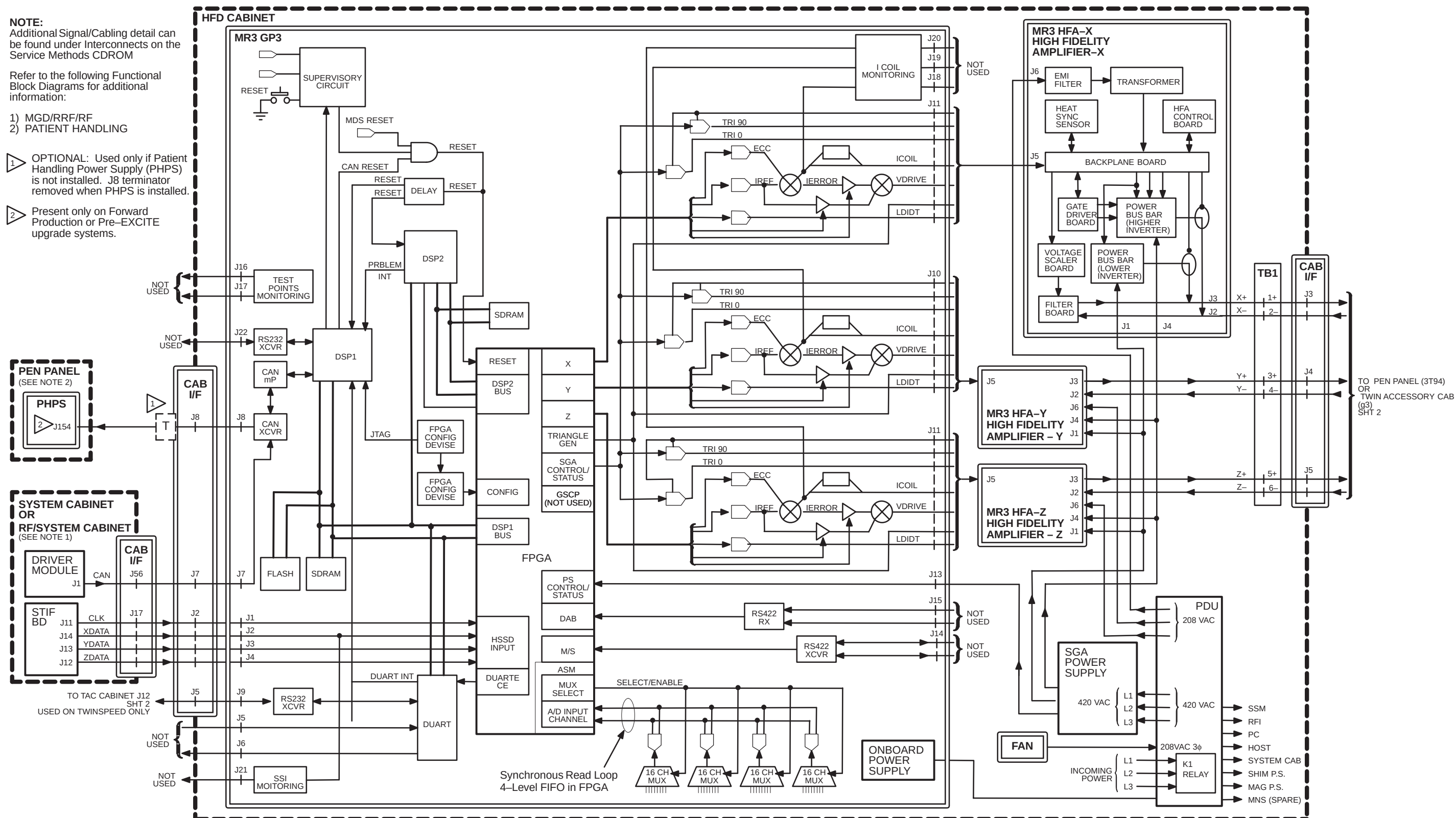
G3 & 3T94 EXCITE HD (12.x) HDx (14.x) & HDxT (15.x) GRADIENT – HFD
