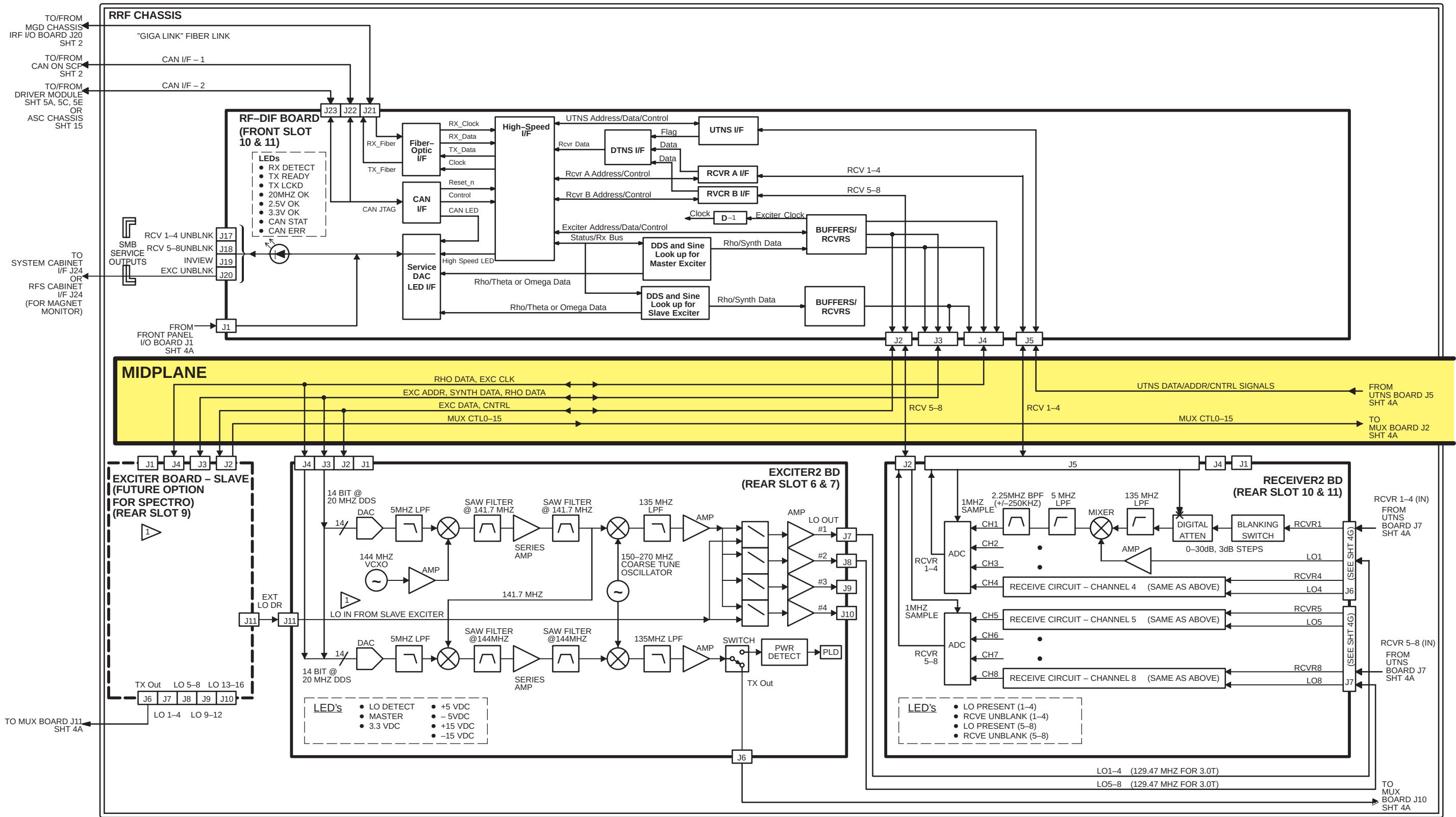
G3 & 3T94 EXCITE HD (12.x), HDx (14.x) & HDxt (15.x) MGD/RRF/RF SUBSYSTEM (8 Channel Systems) RRF CHASSIS INTERCONNECT BLOCK DIAGRAM 1 OF 2A (8 Channel) SHEET 3A OF 18
