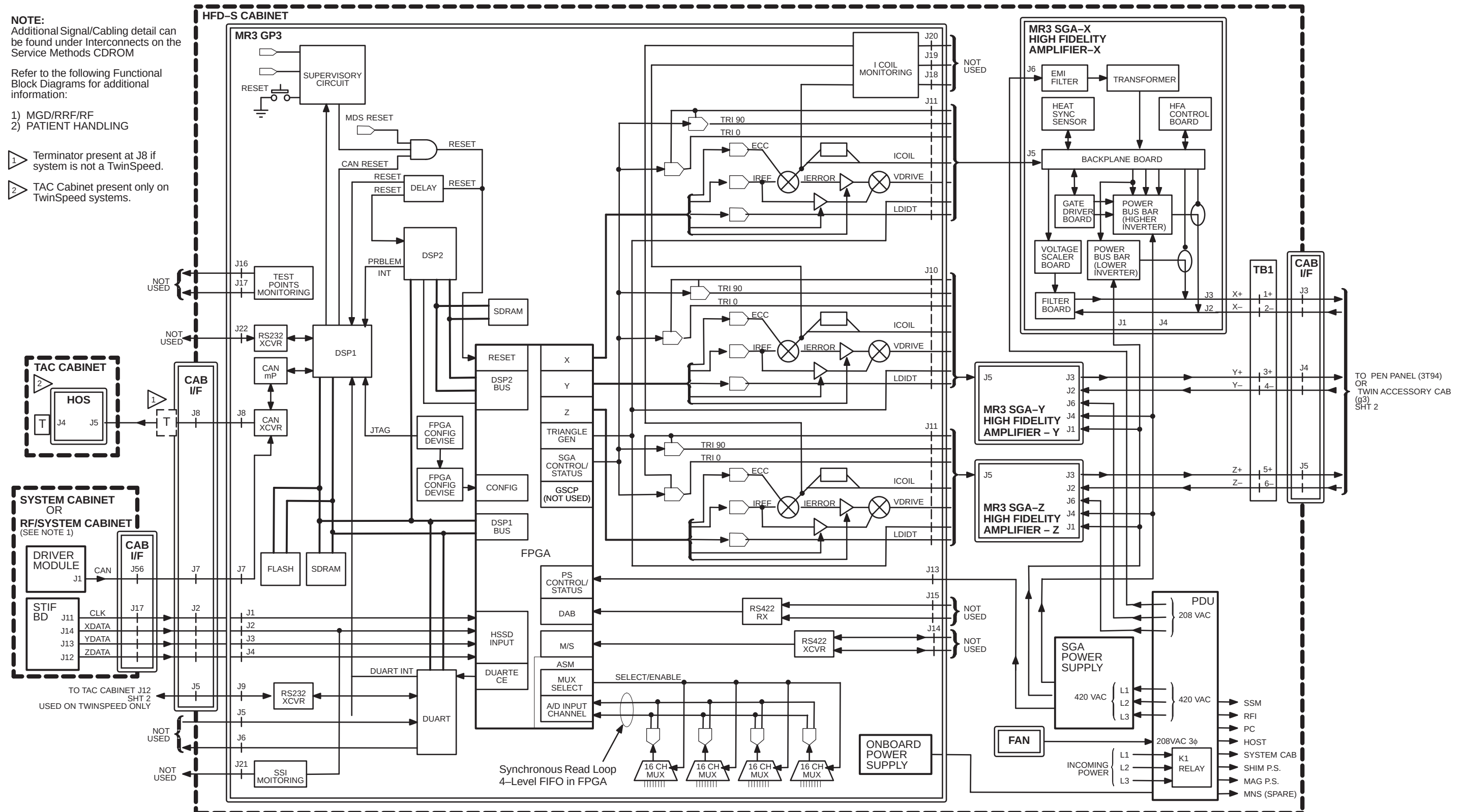
G3 & 3T94 EXCITE HD (12.x), HDx (14.x) & HDxT (15.x) GRADIENT – HFD-S (Upgraded ACGD)
