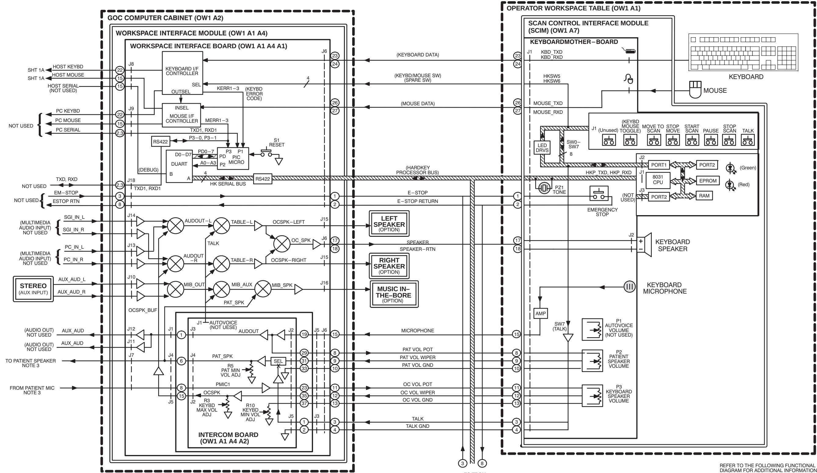
G3 & 3T94 EXCITE HD (12.x) OVERALL SYSTEM (OPERATOR WORKSPACE CABINET/TABLE with WIM) SHEET 2A OF 2
